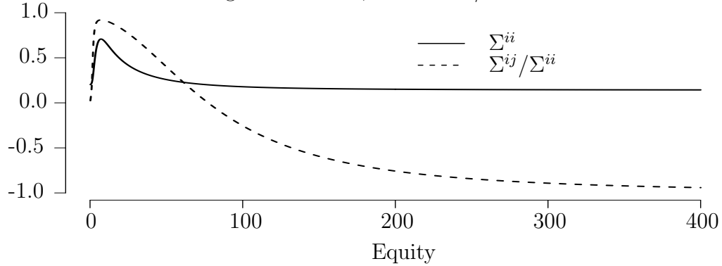
Figure 8: N = 2, \Sigma^{ii} and \Sigma^{ij}/\Sigma^{ii}
