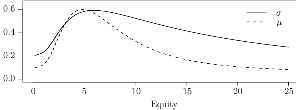
Figure 1: Volatility and mean of the price process
