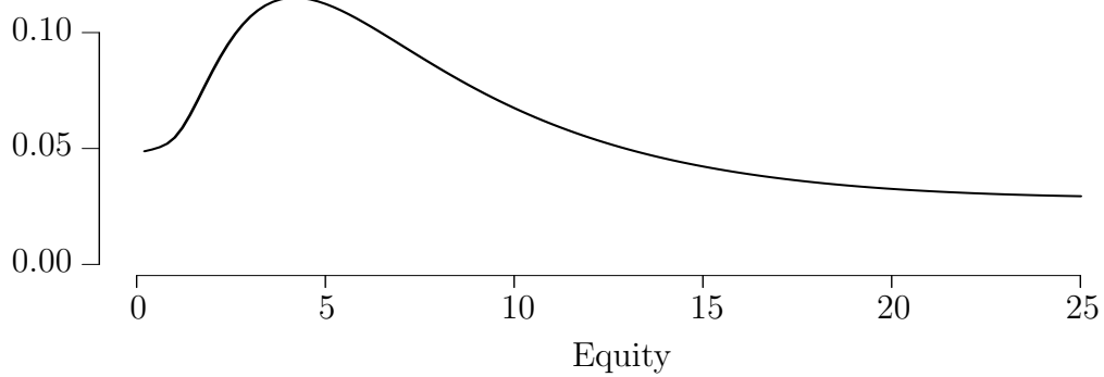
Figure 2: Lagrange Multiplier
