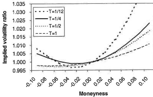
Figure 5 : Implied volatility smile for various maturities
