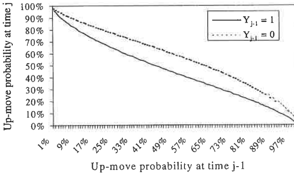
Figure 3 : Up-move probability \pi_j as a function of past probability \pi_{j-1}
