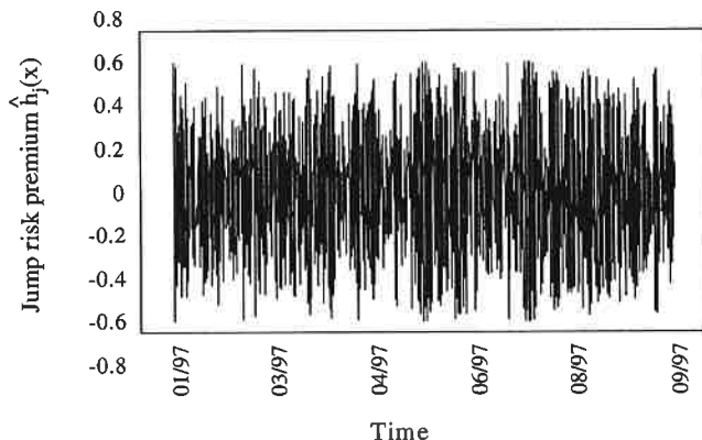
Figure 4 : Evolution of the risk premium \hat{h}_j(x)
