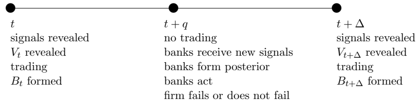
Figure 1: Timing assumptions
