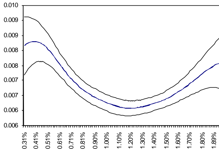
Figure 14: Aaa spread volatility with 95% confidence band
