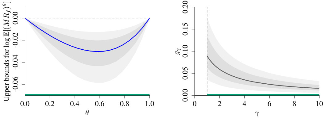
Figure 5: Convexity bounds for \theta \in (0, 1) (left). The attractiveness of investment opportunities, from the perspective of an investor with relative risk aversion \gamma (right). Dark and light gray shaded areas indicate point-wise 68% and 95% confidence intervals.
