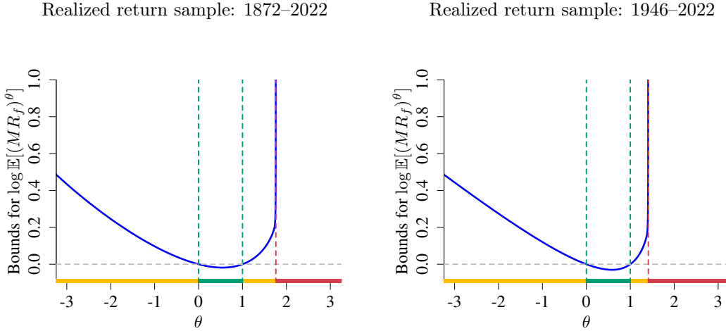
Figure 4: Convexity bounds for the moments of the SDF. The blue curves are lower bounds on SDF moments when \theta < 0 or \theta > 1 and upper bounds when \theta \in (0, 1) . Shading along the axis indicates the green, yellow and red regions as discussed in Section 3.2.
