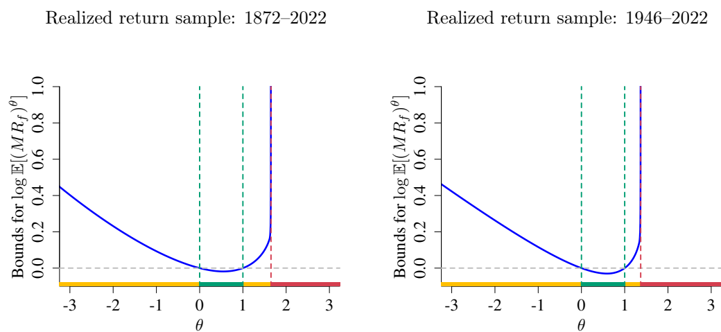
Figure OA.8: Convexity bounds for the moments of the SDF: option sample starting March 6, 2008.
