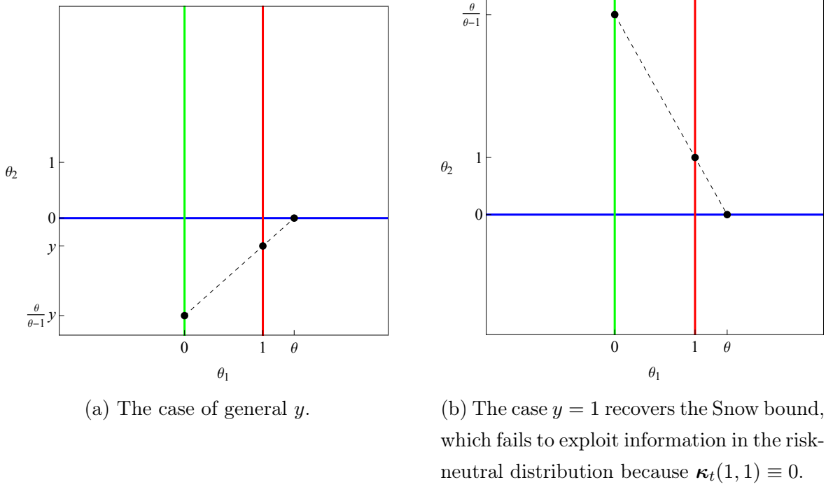
Figure 2: The use of convexity in the proof of Result 1.
