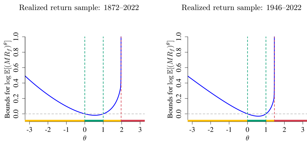
Figure OA.10: Convexity bounds for the moments of the SDF: moneyness filter -6 \leq m \leq 3 applied to the option sample.
