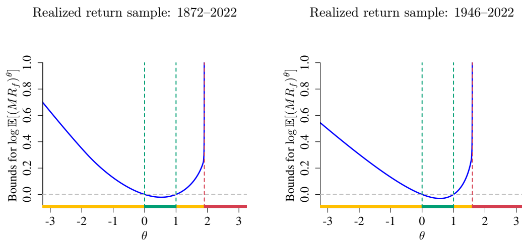
Figure OA.7: Convexity bounds for the moments of the SDF: using daily observations of option prices and realized returns.
