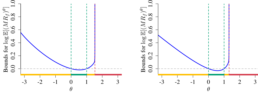
Figure OA.4: Moment bounds calculated using mid-market option prices, extrapolating using a flat volatility smile.
