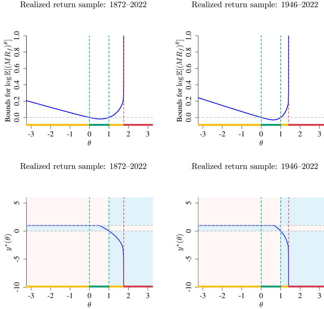
Figure OA.9: Convexity bounds for the moments of the SDF and their optimizing values based on the most conservative approach to extrapolating option offer prices.
