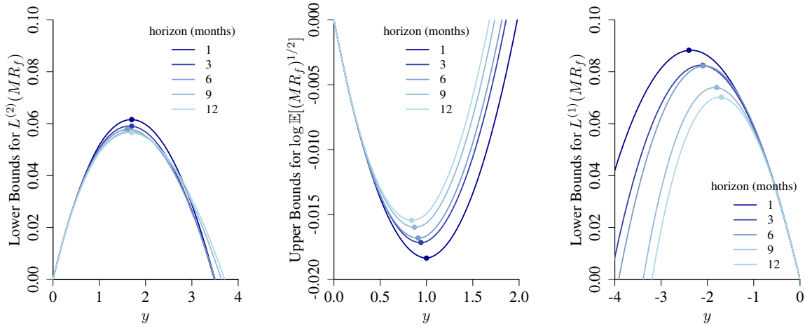
Figure OA.5: Moment bounds are well-behaved for \theta \in (0, 1) and for the two entropy bounds. This figure shows bounds on the \theta = 1/2 moment of the SDF and on the two entropy measures as a function of y across different horizons (annualized). Dots represent the optimizing values of y (which, in the left and right panels, supply the risk aversion measure described in Result 5).
