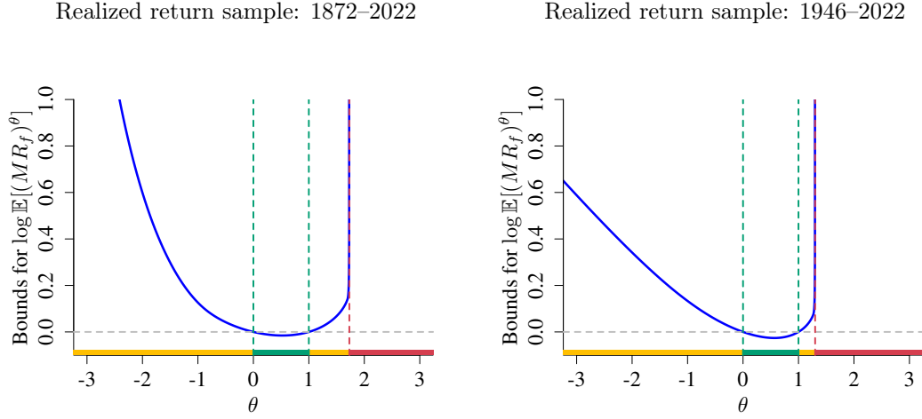
Figure OA.2: Convexity bounds for the moments of the SDF: one-year horizon.
