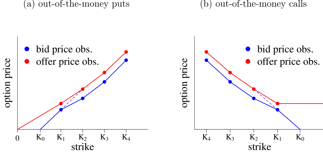
Figure OA.1: Conservative extrapolation of option prices in Section 4.1.
