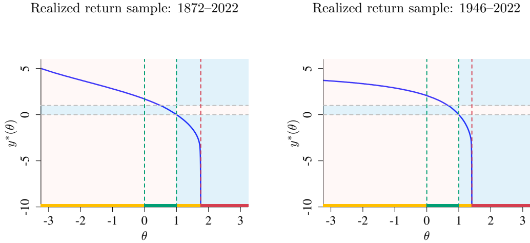
Figure OA.3: Optimizing values for the convexity bounds.
