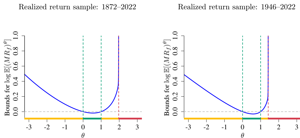
Figure OA.6: Convexity bounds for the moments of the SDF: no extrapolation outside the range of observed option strikes.
