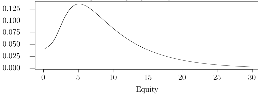
Figure 2: Lagrange Multiplier
