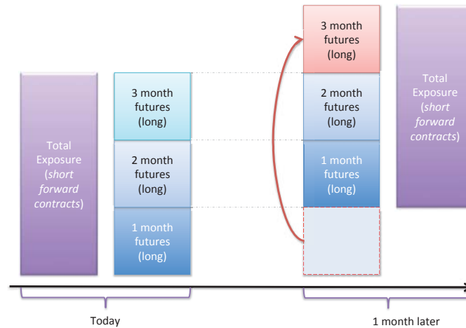
Figure 8: Stack hedging
